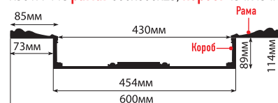
KS61A-115 (600x600x114)
