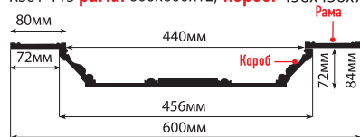
KS61-115 (600x600x84)
