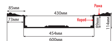
KS61A-937 (600x600x114)
