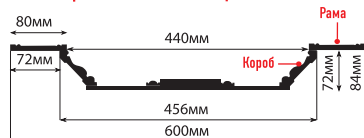
KS61-552 (600x600x84)
